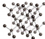
diamond
