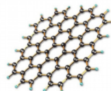
graphene
